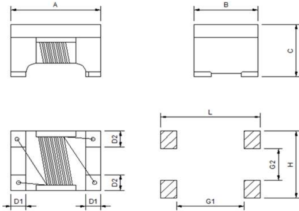
Recommended layout
