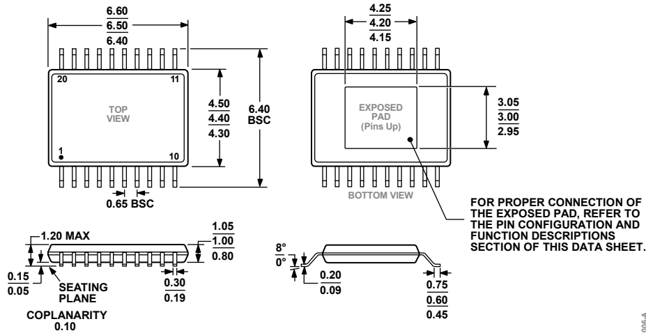
COMPLIANT TO JEDEC STANDARDS MO-153-ACT Figure 53. 20-Lead Thin Shrink Small Outline With Exposed Pad [TSSOP_EP] (RE-20-1) Dimensions shown in millimeters
