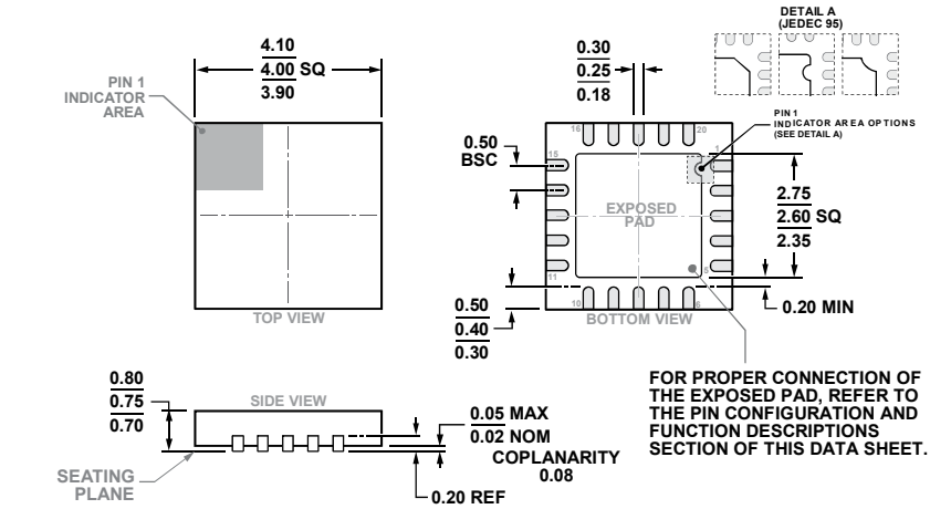
COMPLIANT TO JEDEC STANDARDS MO-220-WGGD-11. Figure 52. 20-Lead Lead Frame Chip Scale Package [LFCSP] 4 mm × 4 mm Body and 0.75 mm Package Height (CP-20-8) Dimensions shown in millimeters
