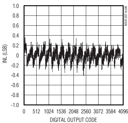
INTEGRAL NONLINEARITY
