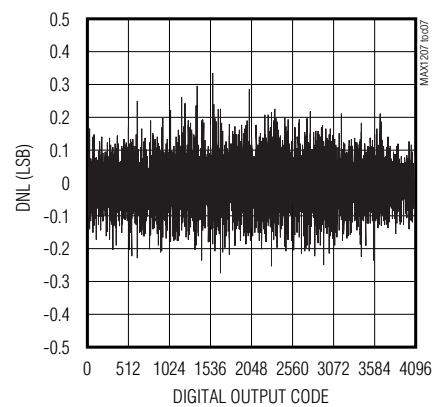
DIFFERENTIAL NONLINEARITY
