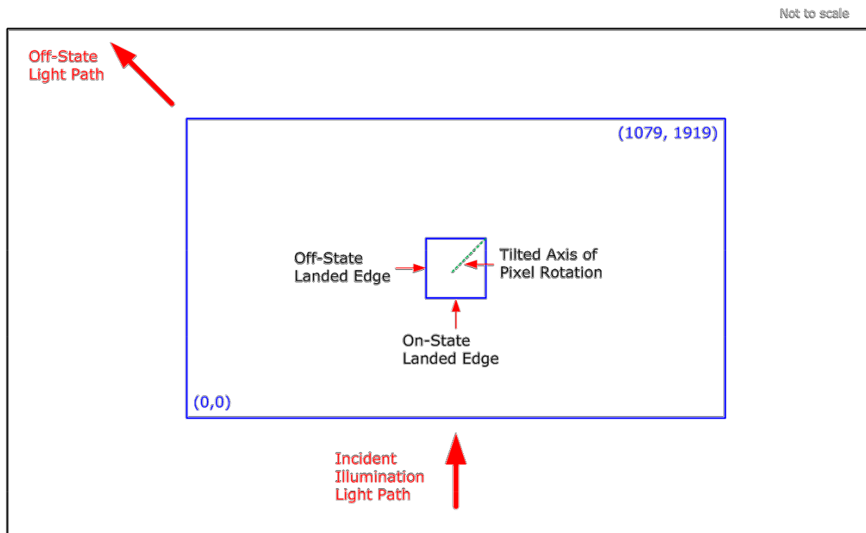
Figure 17. Landed Pixel Orientation and Tilt
