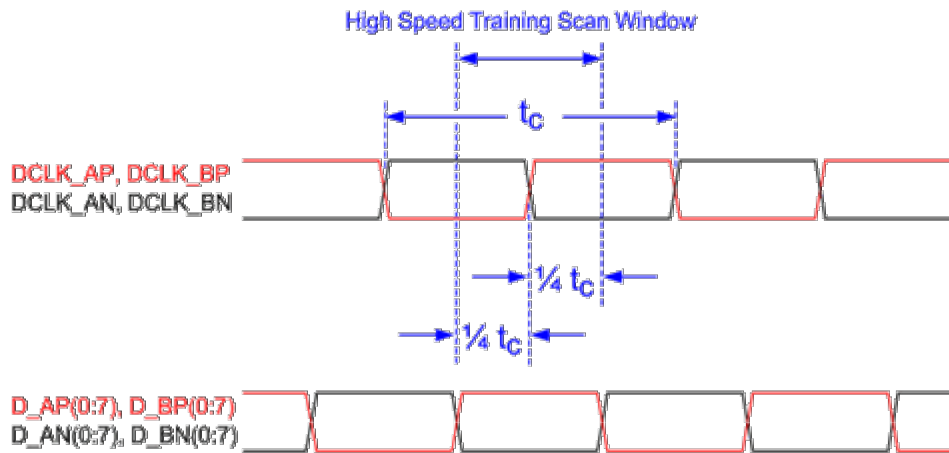
Figure 7. High-Speed Training Scan Window
