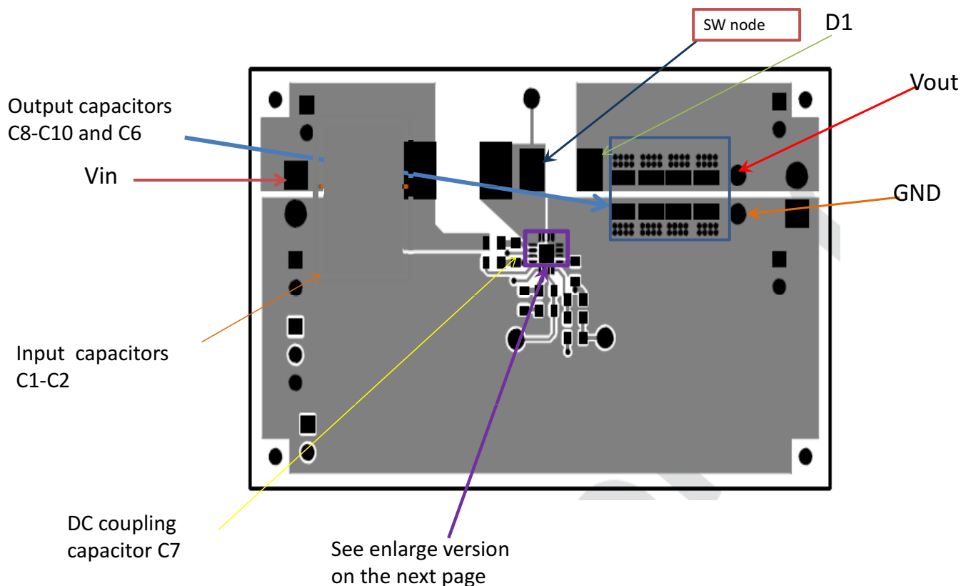
Figure 11-1. TPS55340 Top-Side Layout
