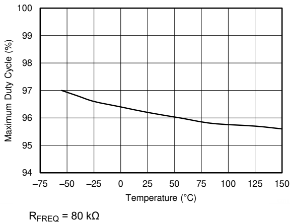
Figure 7-11. Maximum Duty Cycle vs Temperature
