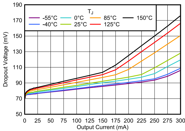
Figure 6-31. Dropout Voltage vs I_{OUT}
