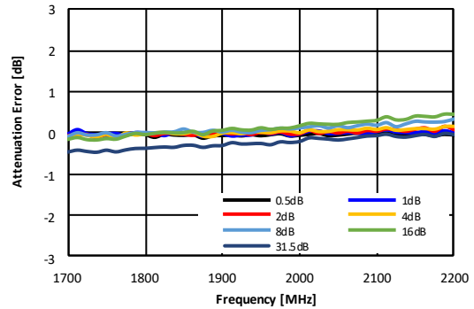
Figure 54. Attenuation Error vs Frequency over Major Attenuation Setting(DSA2 Control, DSA1 Att Setting 0dB @+25°C)
