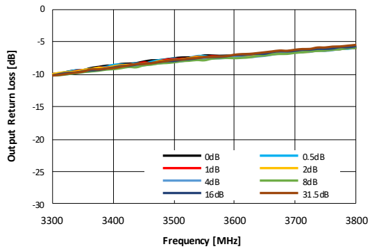
Figure 105. Output Return Loss vs Frequency
