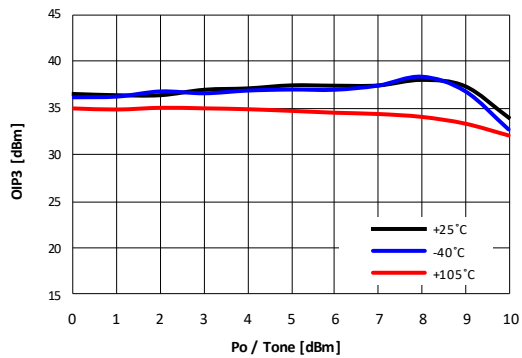
Figure 107. OIP3 vs Output Power
