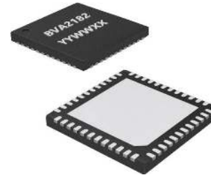
48-lead 7mm x 7mm x 0.9mm QFN
