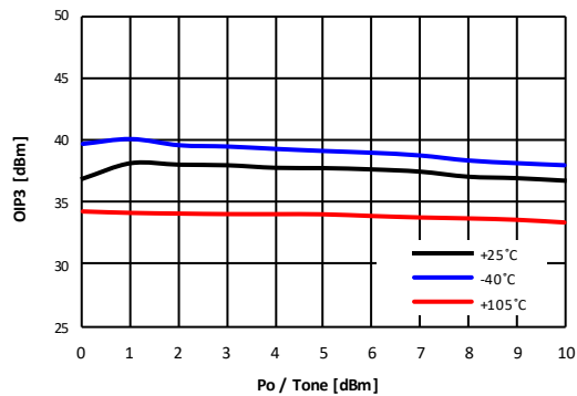
Figure 17. OIP3 vs Output Power over Temperature(@0.6GHz, DSA1,2 Att Setting 0dB)
