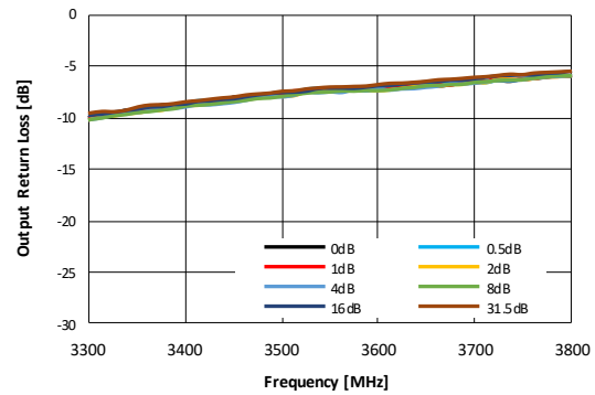
Figure 106. Output Return Loss vs Frequency
