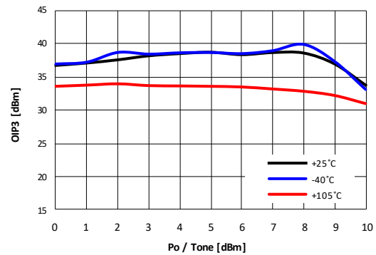
Figure 108. OIP3 vs Output Power
