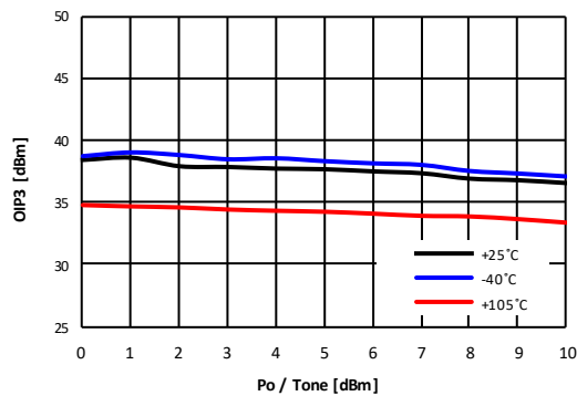
Figure 19. OIP3 vs Output Power over Temperature(@1GHz, DSA1,2 Att Setting 0dB)
