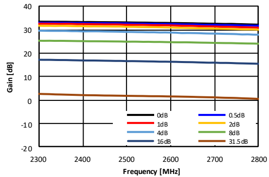
Figure 67. Gain vs Attenuation Settings over Major Attenuation Setting(DSA2 Att Setting 0dB, DSA1 Att Control)
