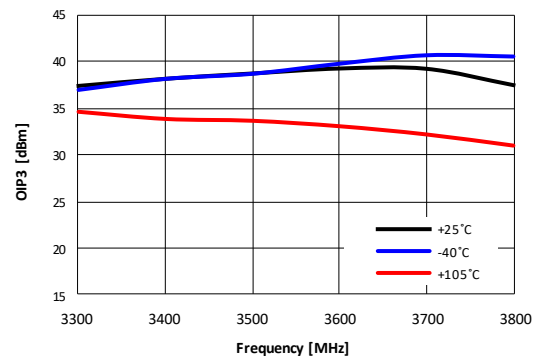
Figure 110. OIP3 vs Frequency
