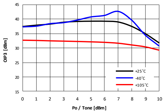
Figure 109. OIP3 vs Output Power
