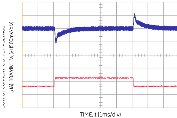
Figure 3. Transient Response to Dynamic Load Change from 25% to 50% to 25% of Full Load at Room Temperature and 48 Vdc Input; 0.1A/µS ; C o,ext = 470µF.
