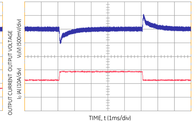
Figure 6. Transient Response to Dynamic Load Change from 50% to 75% to 50% of Full Load at Room Temperature and 48 Vdc Input; 0.1A/µS ; C o,ext = 470µF.
