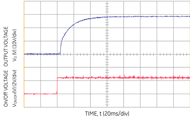
Figure 4. Typical Start-Up Using Remote On/Off, R1=30Kohm; C o,ext = 470µF.
