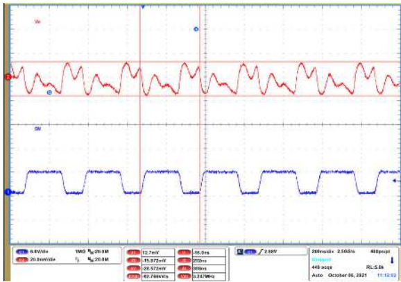
Figure 9-74. Input Voltage Ripple
