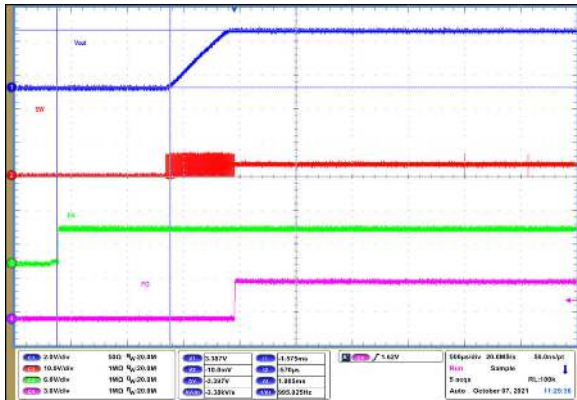
Figure 9-62. Start-Up Timing
