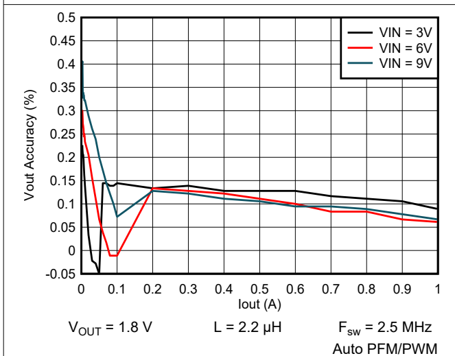
Figure 9-30. Output Voltage vs Output Current
