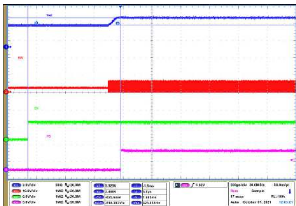
Figure 9-62. Start-Up Timing
