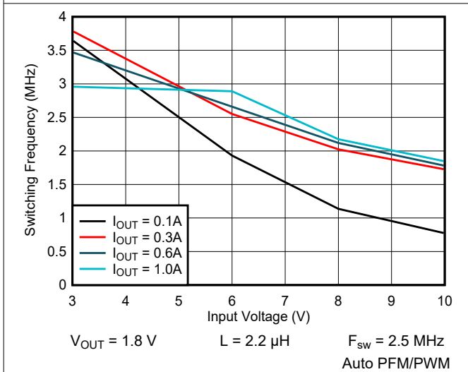
Figure 9-28. Switching Frequency vs Input Voltage
