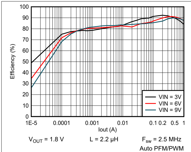
Figure 9-26. Efficiency vs Output Current
