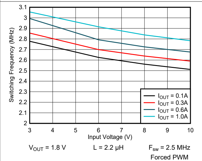
Figure 9-29. Switching Frequency vs Input Voltage
