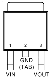
TO-252
