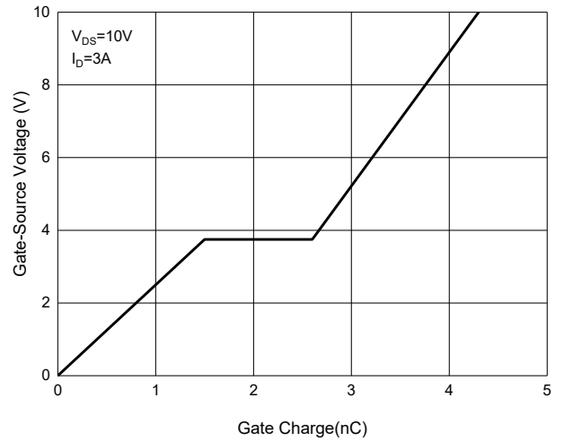
Fig. 4 - Gate Charge
