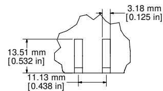
DETAIL FF
