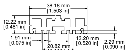
DETAIL GG
