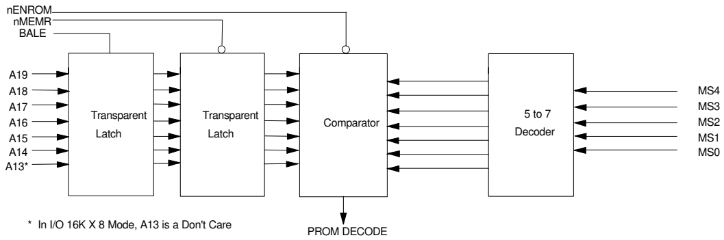
FIGURE 5 - PROM SELECTOR
