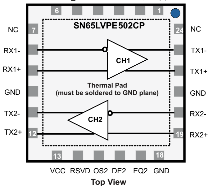
Figure 8. Flow-Through Pin-Out
