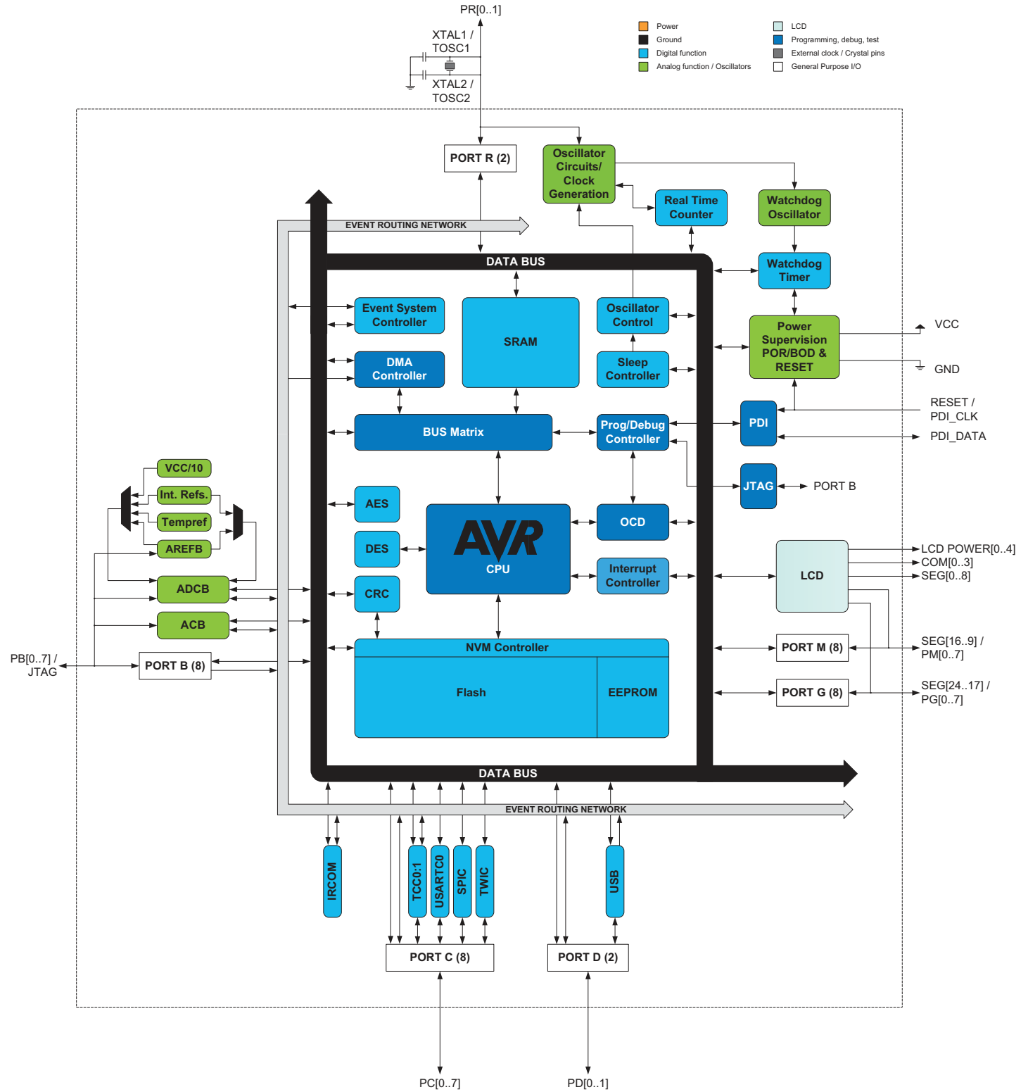
Figure 3-1. XMEGA B3 Block Diagram
