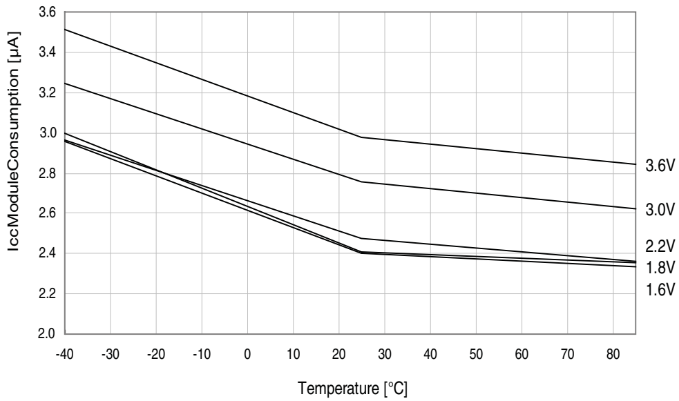
Figure 37-83. Psave vs. Temperature
