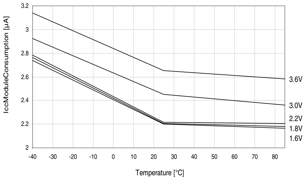
Figure 37-81. I_{CC} LCD LP 32Hz vs. Temperature
