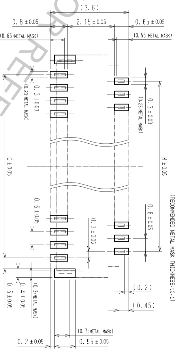
RECOMMENDED LAND PATTERN (SCALE:FREE)
