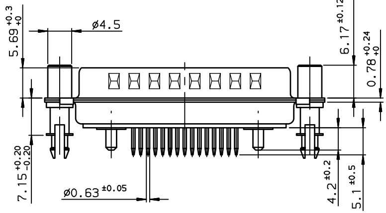
LAYOUT DIMENSIONS (after plating) CONNECTOR SIDE VIEW
