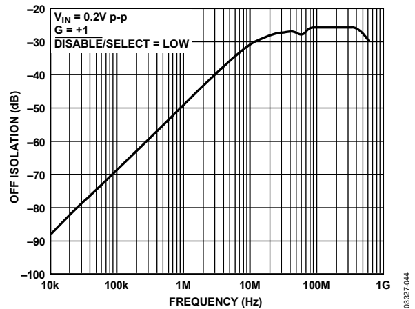
Figure 49. Off Isolation vs. Frequency
