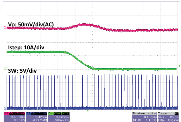
Fig. 37 - SiC451 Load Step, 12.5 A to 0 A, 1 A/ \mu\text{s} , t = 10\text{ }\mu\text{s}/\text{div}
