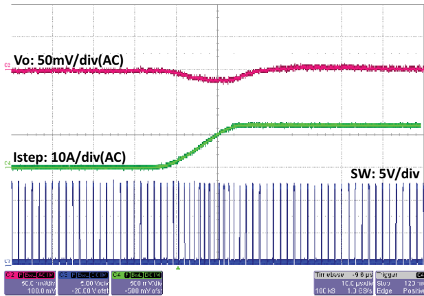
Fig. 34 - SiC451 Load Step, 12.5 A to 25 A, 10 A/ \mu\text{s} , t = 10\text{ }\mu\text{s}/\text{div}
