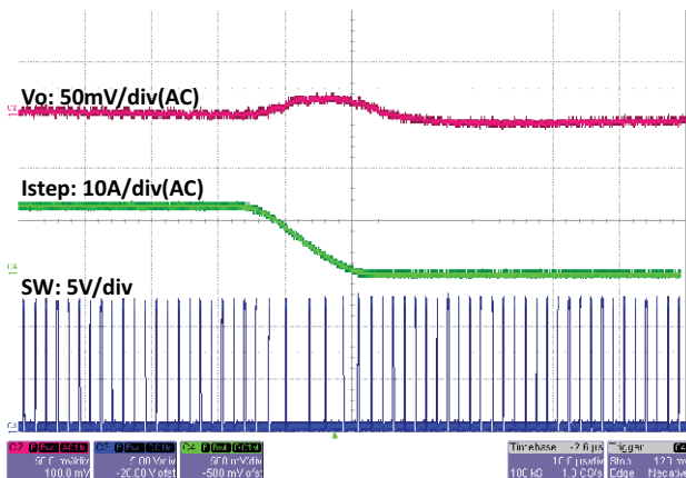
Fig. 35 - SiC451 Load Step, 25 A to 12.5 A, 1 A/ \mu\text{s} , t = 10\text{ }\mu\text{s}/\text{div}
