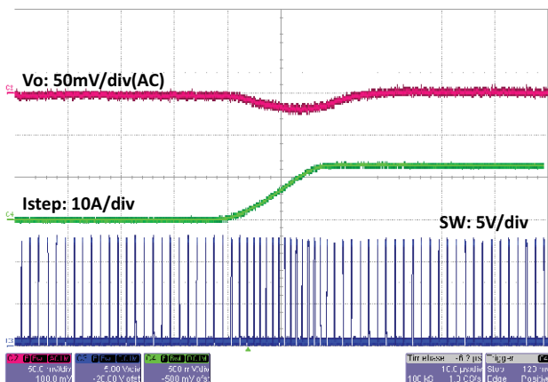
Fig. 36 - SiC451 Load Step, 0 A to 12.5 A, 1 A/ \mu\text{s} , t = 10\text{ }\mu\text{s}/\text{div}
