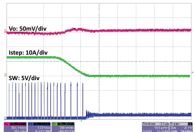
Fig. 39 - SiC451 Load Step, 12.5 A to 0 A, 1 A/ \mu\text{s} , t = 10\text{ }\mu\text{s}/\text{div} Skip Mode Enabled
