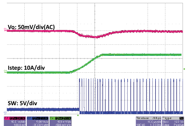
Fig. 38 - SiC451 Load Step, 0 A to 12.5 A, 1 A/ \mu\text{s} , t = 10\text{ }\mu\text{s}/\text{div} Skip Mode Enabled
