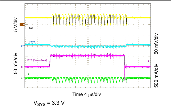
Figure 10-35. 3.3 V SYS Load Transient, 0 to 50 mA
