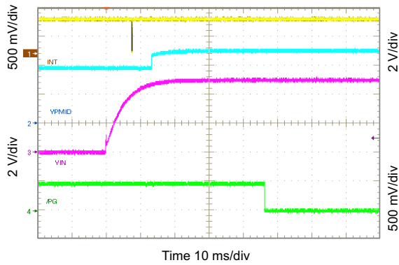
Figure 10-57. Show \overline{PG} and \overline{INT} Timing ( V_{IN} Insertion)
