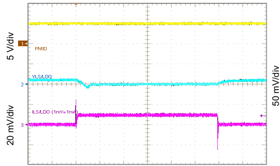
V_{LSLDO} = 0.8 \text{ V} Figure 10-45. 0.8 V LSLDO Load Transient, 0 to 10 mA
