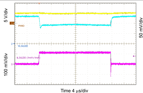
Figure 10-52. 1.8 V L SLDO Load Transient, 0 to 100 mA
