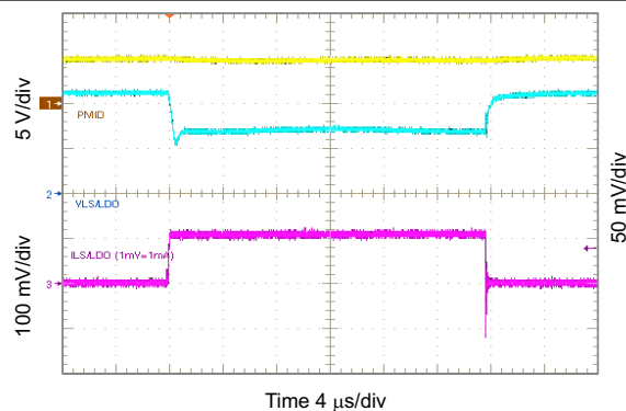
Figure 10-51. 1.2 V L SLDO Load Transient, 0 to 100 mA
