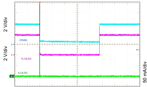
Figure 10-43. Short Circuit and Recovery for LS
