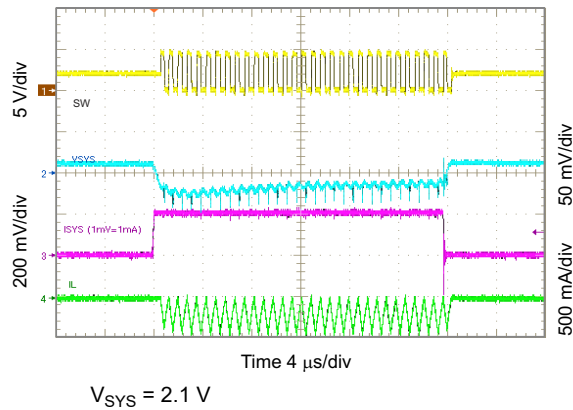
Figure 10-38. 2.1 V SYS Load Transient, 0 to 200 mA
