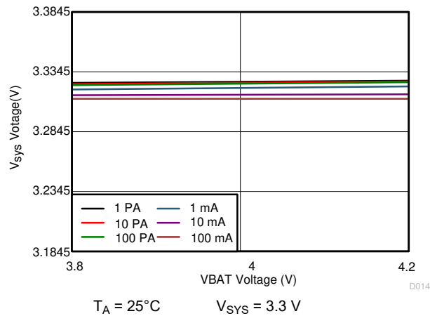
Figure 10-22. 3.3 V sys Line Regulation
