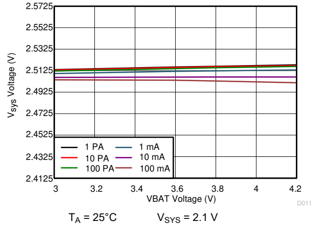
Figure 10-21. 2.1 V sys Line Regulation
