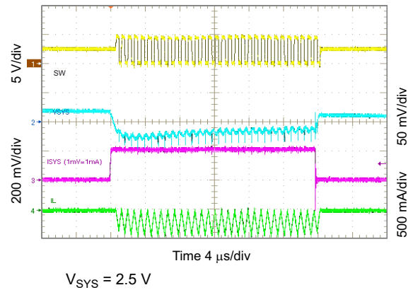
Figure 10-39. 2.5 V SYS Load Transient, 0 to 200 mA
