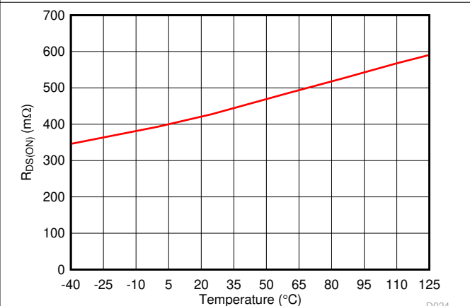
Figure 8-6. Blocking FET R_{DS(ON)} vs Temperature
