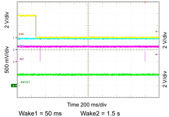
Figure 10-62. Show \overline{MR} Timing
