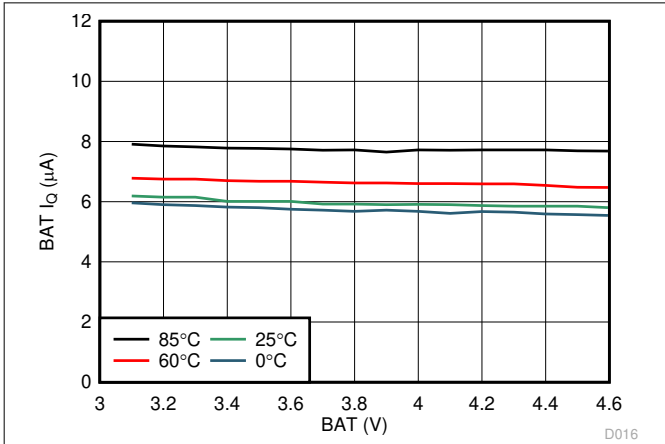
Figure 8-3. Active BAT, I_Q
