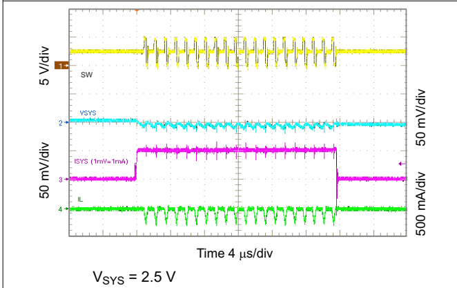
Figure 10-34. 2.5 V SYS Load Transient, 0 to 50 mA
