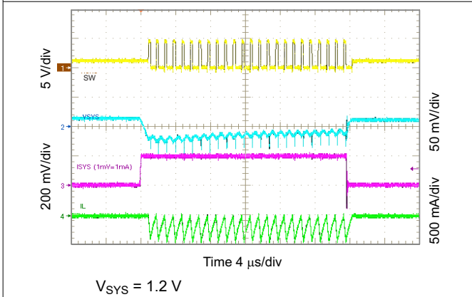
Figure 10-36. 1.2 V SYS Load Transient, 0 to 200 mA
