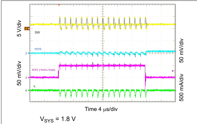
Figure 10-32. 1.8 V SYS Load Transient, 0 to 50 mA
