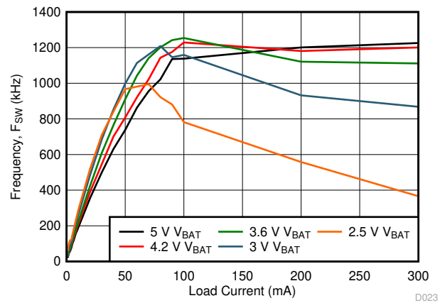
Figure 10-23. 1.8 V sys Switching Frequency vs Load Current
