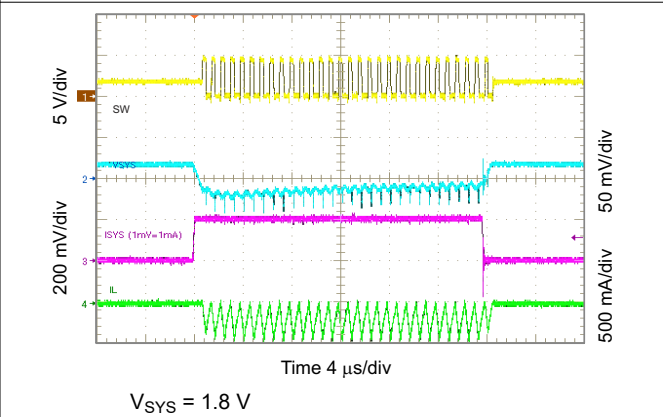
Figure 10-37. 1.8 V SYS Load Transient, 0 to 200 mA
