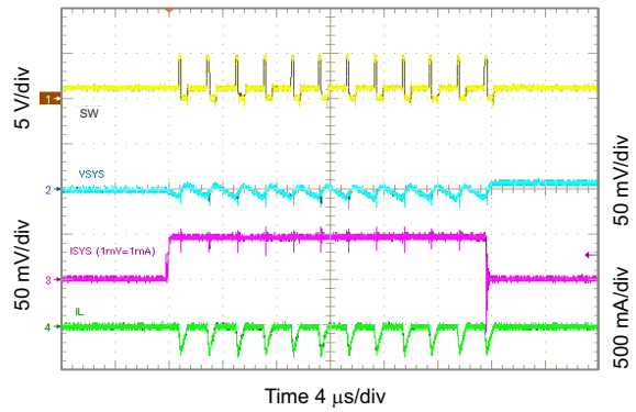
Figure 10-31. 1.2 V_{SYS} Load Transient, 0 to 50 mA
