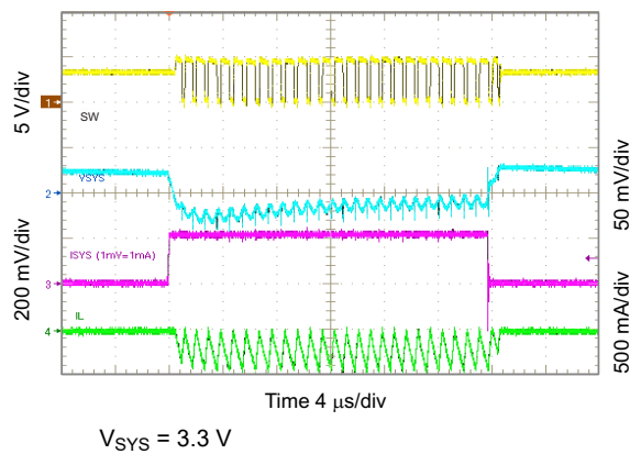
Figure 10-40. 3.3 V SYS Load Transient, 0 to 200 mA
