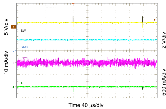
Figure 10-22. 3.3 V sys Line Regulation
