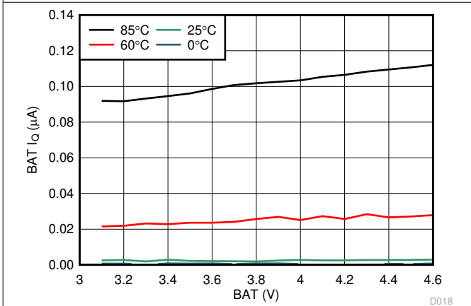
Figure 8-5. Ship Mode BAT, I_Q
