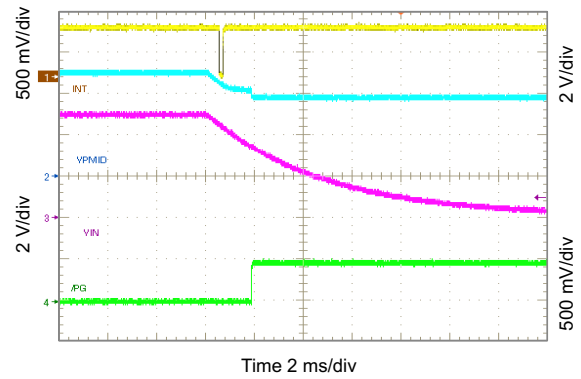
Figure 10-58. Show \overline{PG} and \overline{INT} Timing ( V_{IN} Removal)
