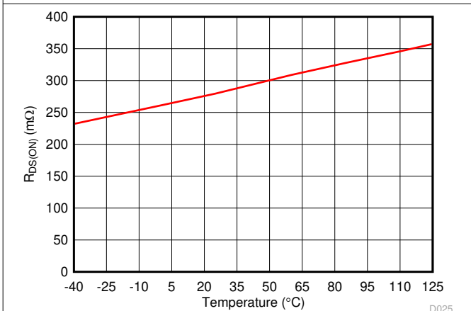
Figure 8-7. Battery Discharge FET R_{DS(ON)} vs Temperature
