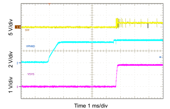
Figure 10-41. Startup Showing SS on SYS in PWM Mode
