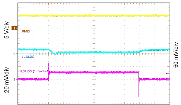
V_{LSLDO} = 2.5 \text{ V} Figure 10-48. 2.5 V LSLDO Load Transient, 0 to 10 mA
