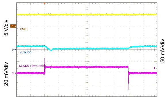
V_{LSLDO} = 1.8 \text{ V} Figure 10-47. 1.8 V LSLDO Load Transient, 0 to 10 mA
