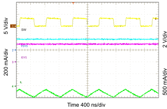
Figure 10-30. Light Load Operation Showing SW
