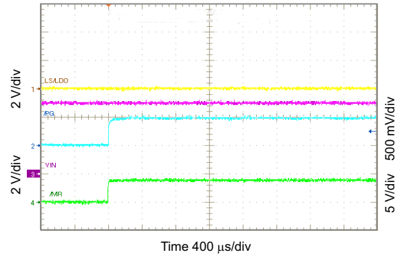
Figure 10-60. \overline{PG} Functions as Shifted \overline{MR} Output
