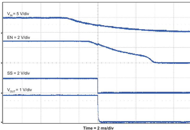
Figure 11. TPS5432EVM-116 Shut Down Relative to V IN
