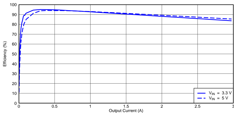
Figure 1. TPS5432EVM-116 Efficiency
