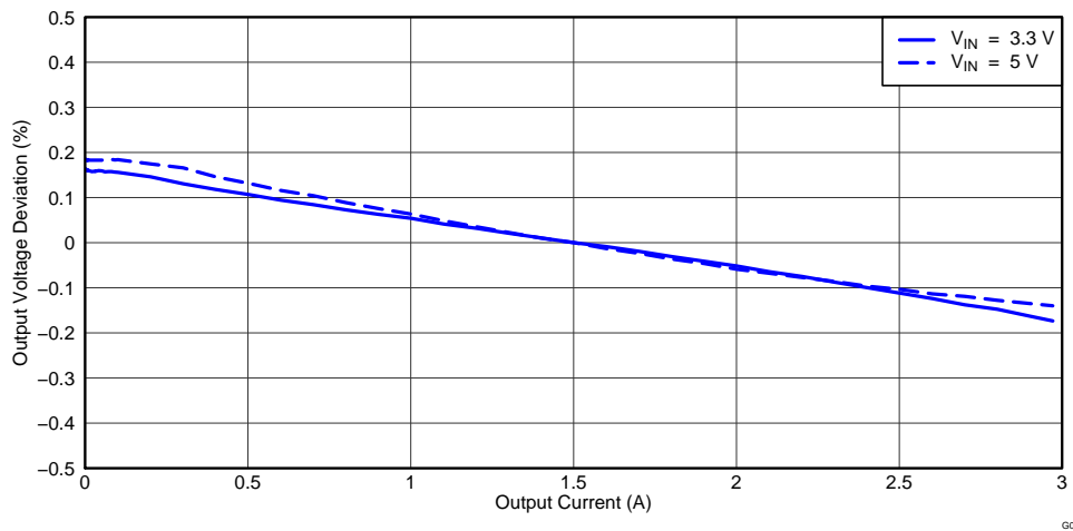
Figure 3. TPS5432EVM-116 Load Regulation
