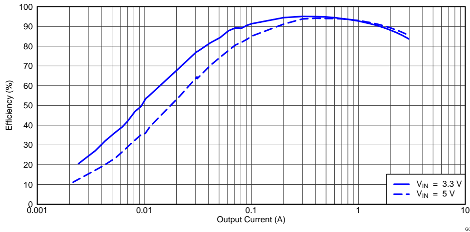
Figure 2. TPS5432EVM-116 Low Current Efficiency
