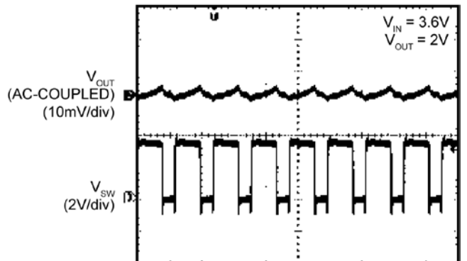
Switching Waveform Continuous Mode (2A)
