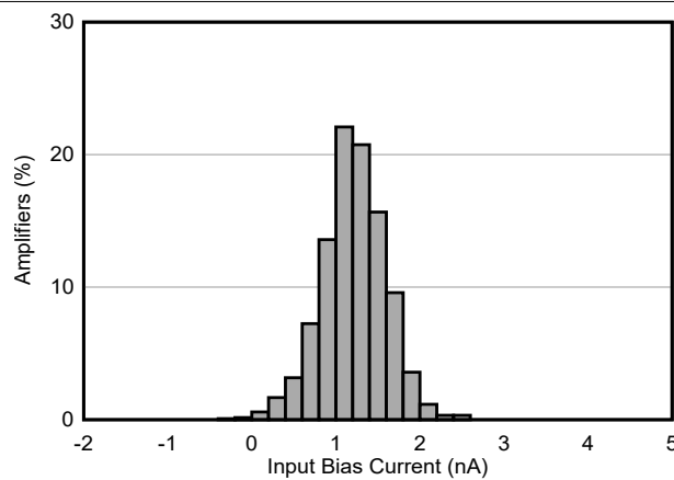
Figure 7-5. Typical Distribution of Inverting Input Bias Current
