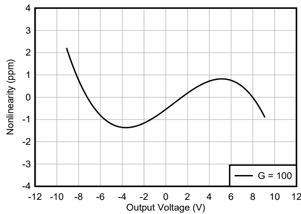
Figure 7-39. Gain Nonlinearity
