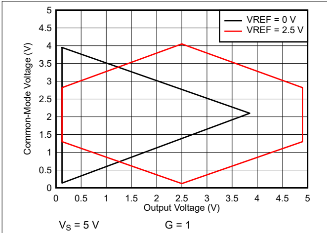
Figure 7-55. Input Common-Mode Voltage vs Output Voltage
