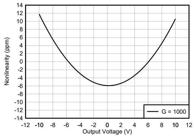
Figure 7-40. Gain Nonlinearity
