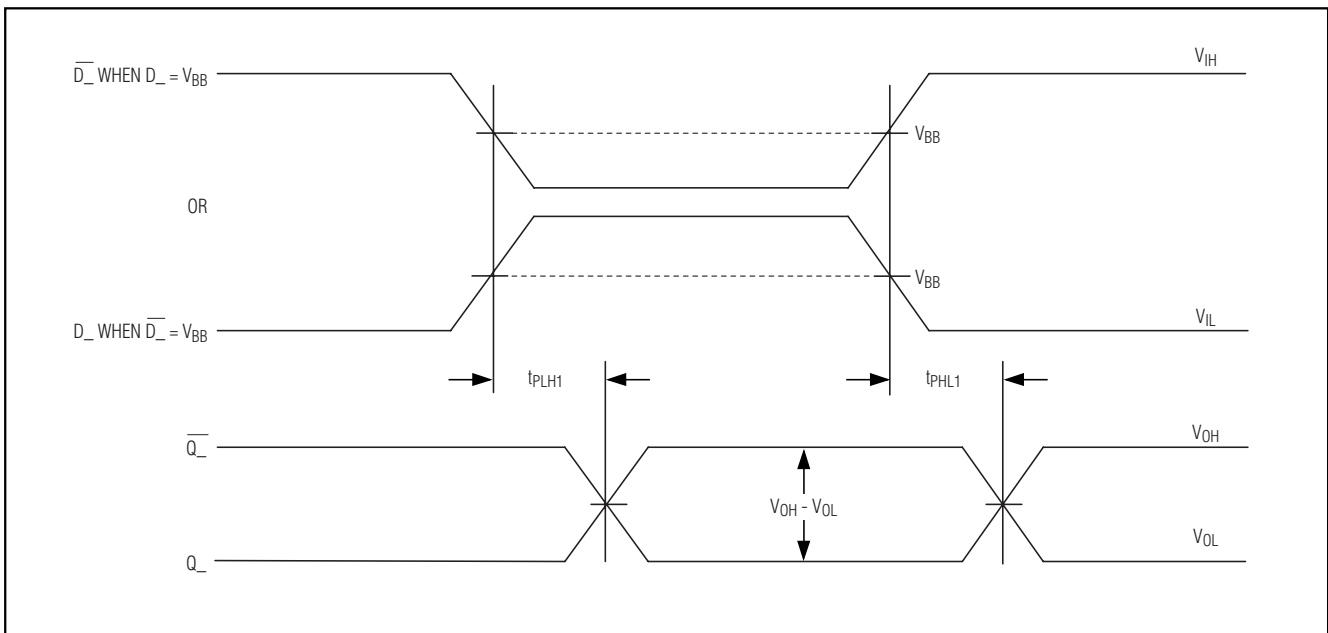
Figure 3. Single-Ended Input-to-Output Propagation Delay Timing Diagram
