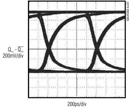
DIFFERENTIAL OUTPUT EYE PATTERN AT 1Gbps, PRBS 2 23 - 1, NRZ DATA PATTERN
