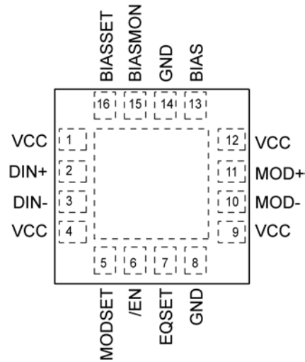
16-Pin QFN
