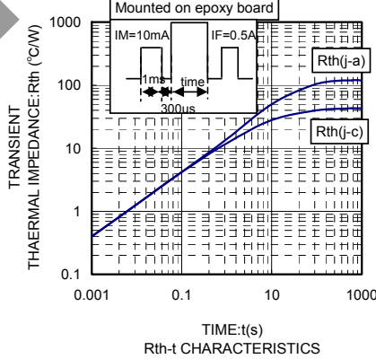
Rth-t CHARACTERISTICS
