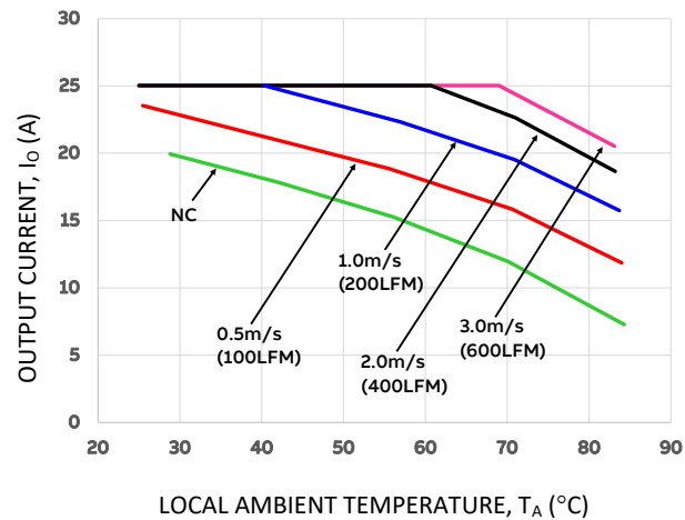
Figure 22. Output Current Derating for the Base Plate EBDW025A0Bxx-H and 0.25" heat sink in the Transverse Orientation; Airflow Direction from Vin(-) to Vin(+); Vin = 48V.
