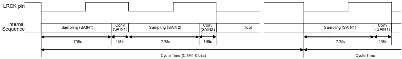
Figure 59. SAR Control Sequence (SA2 bit = "1")
