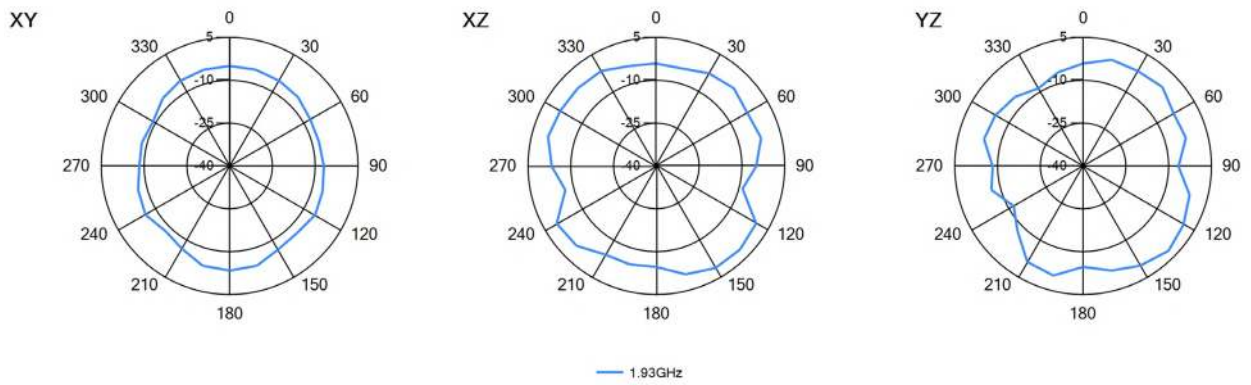
3D pattern at 1930MHz
