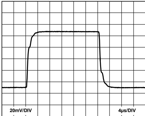
Figure 52. Small Signal Pulse Response, R_L = 10\text{ k}\Omega , C_L = 100\text{ pF} , G = 10
