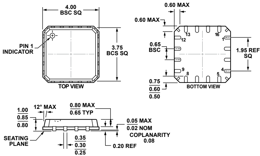
Figure 73. 16-Lead Lead Frame Chip Scale Package [LFCSQ_VQ] 4 mm × 4 mm Body, Very Thin Quad, with Hidden Paddle (CP-16-19) Dimensions shown in millimeters
