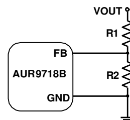
Figure 30. Setting the Output Voltage
