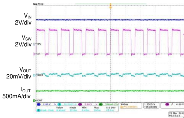
Time 800ns/div
