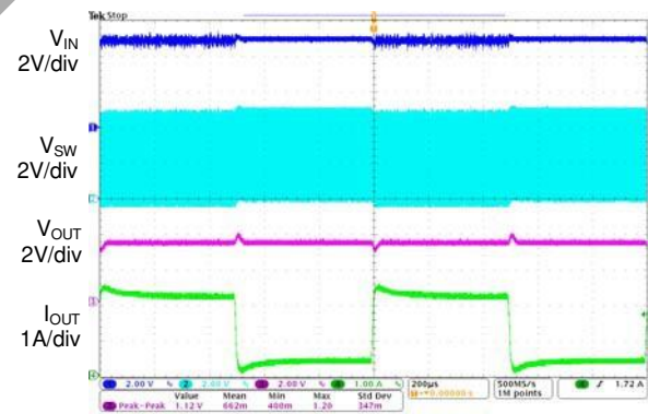
Time 200µs/div
