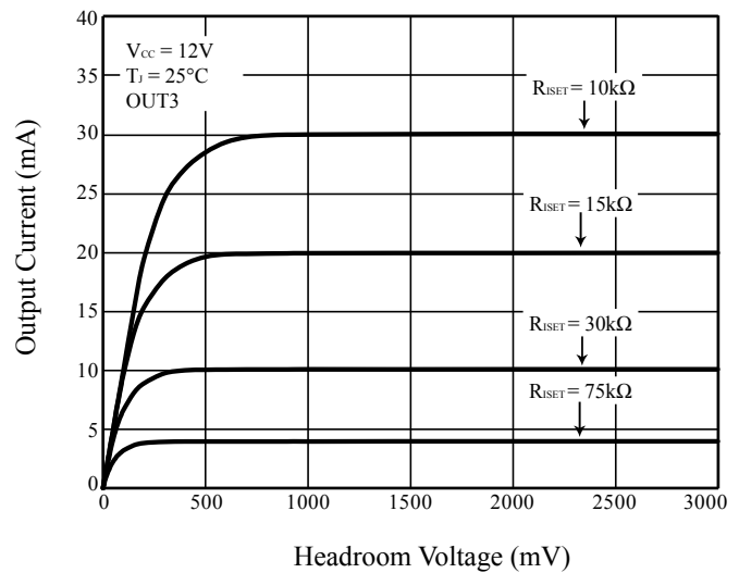
Figure 28 Output Current 3 vs. Headroom Voltage
