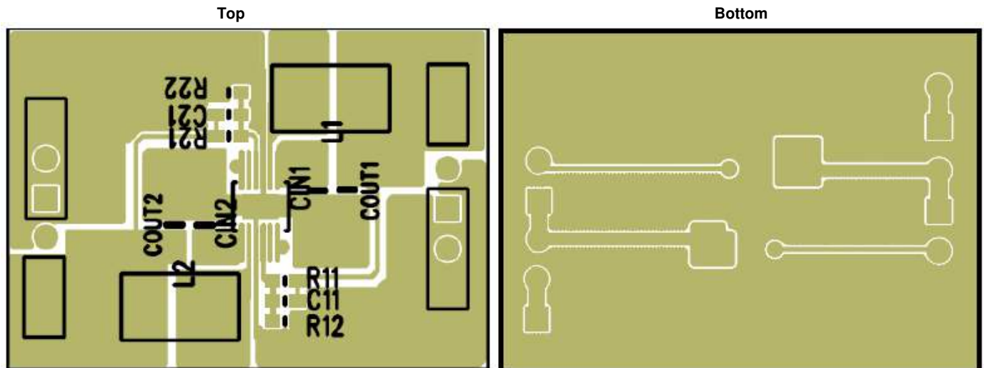
Figure 3. PAM2306 Suggested Layout
