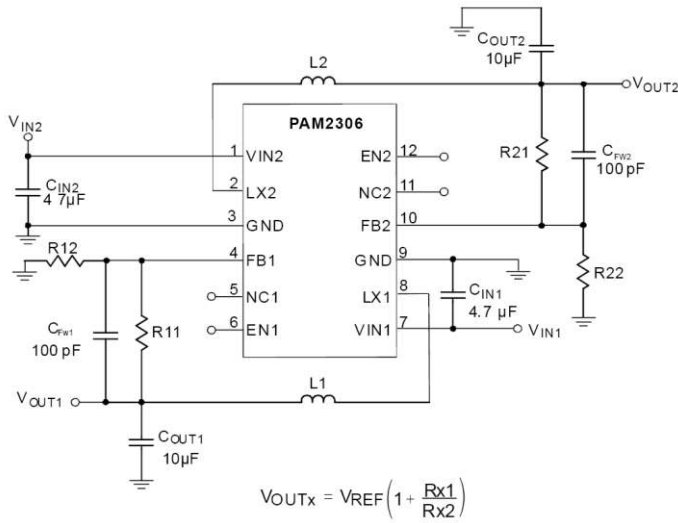
Figure 1. Adjustable Voltage Regulator
