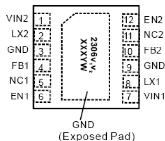
W-DFN3030-12 (Type US)
