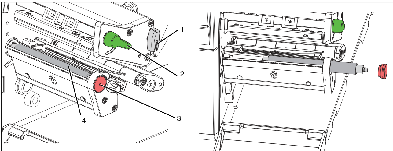
Figure 4-3 Removing and fitting the pressure roller
