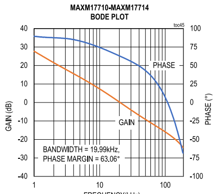
CONDITIONS: PWM MODE, V_{OUTB} = 3.3V , I_{OUTB} = 150mA , f_{SW} = 375kHz
