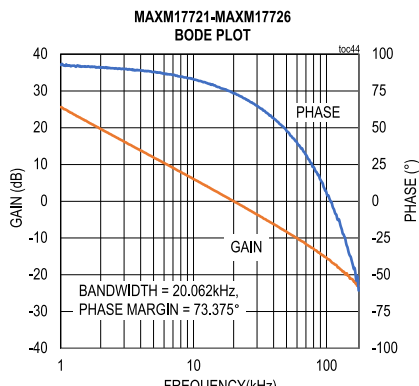
CONDITIONS: PWM MODE, V_{OUTB} = 2.5V , I_{OUTB} = 150mA , f_{SW} = 350kHz
