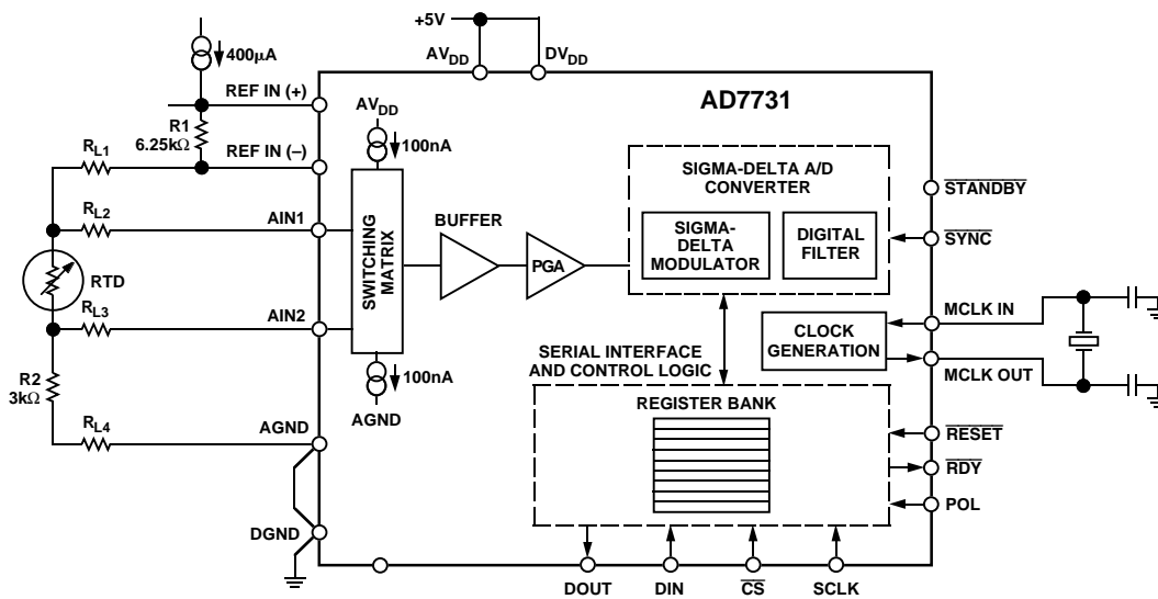
Figure 24. RTD Measurement Using the AD7731
