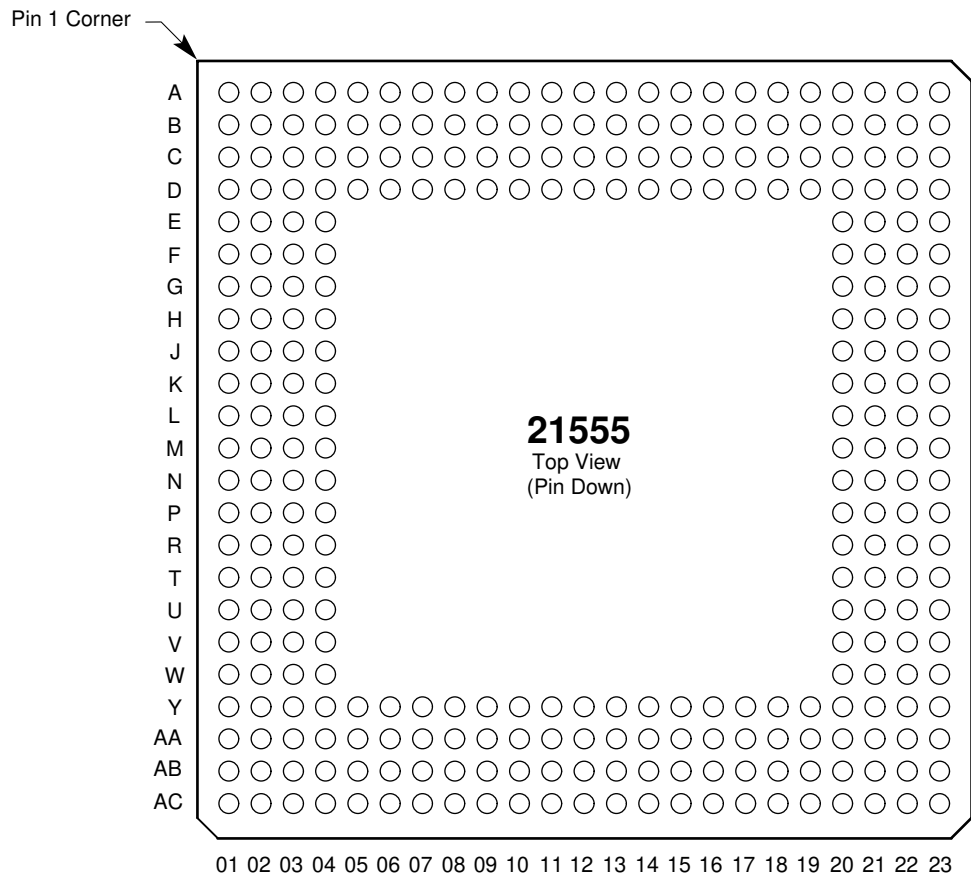
Figure 3. 21555 PBGA Cavity Down View
