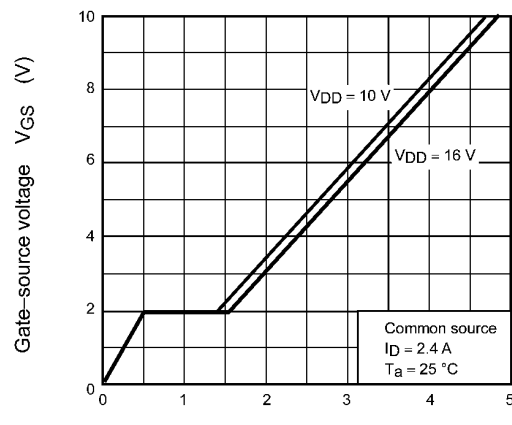
Fig. 8.12 Dynamic Input Characteristics
