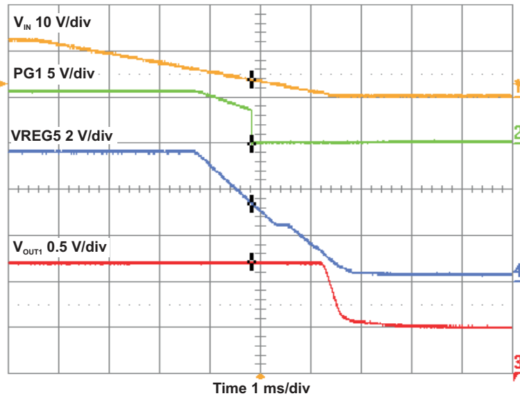
Figure 4-17. TPS54294EVM Converter 1 Shut-Down Relative to V_{IN}
