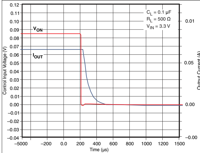
Figure 21. t_{OFF} Response
