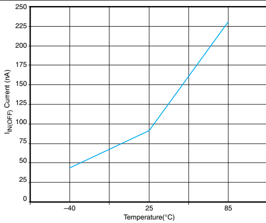
Figure 7. I_{IN(OFF)} vs Temperature ( V_{IN} = 3.3\text{ V} )
