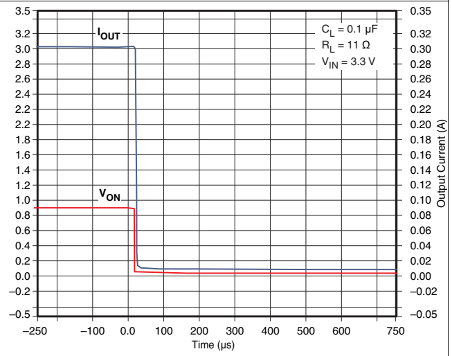
Figure 22. t_{OFF} Response
