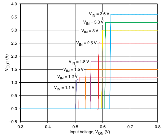
Figure 10. ON-Input Threshold
