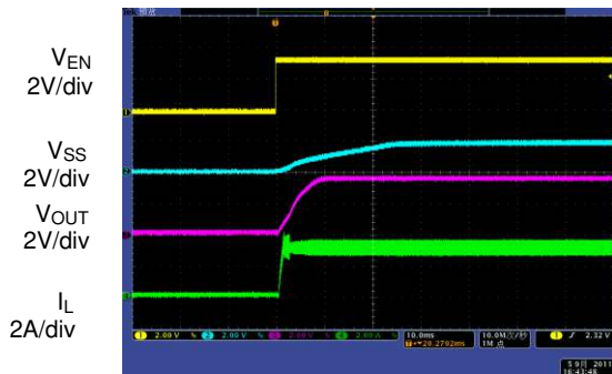
Time 10ms/div
