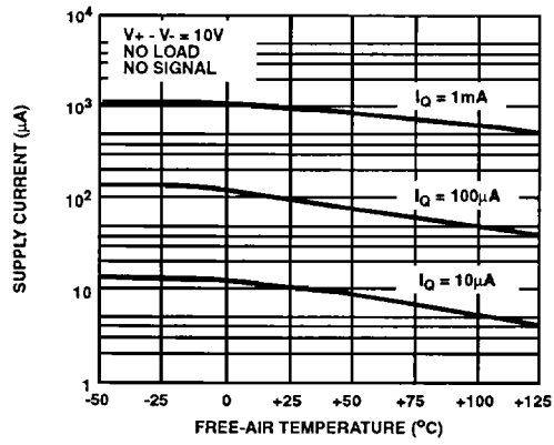
FIGURE 2. SUPPLY CURRENT PER AMPLIFIER vs FREE-AIR TEMPERATURE
