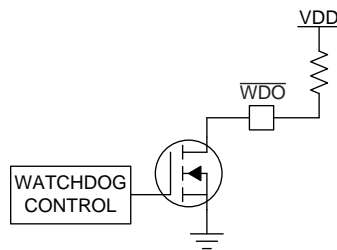
Figure 10. Open-Drain \overline{WDO} Configuration
