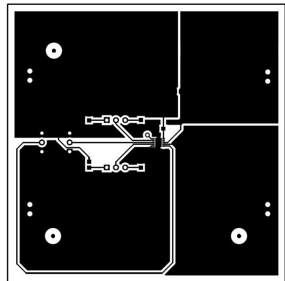
Figure 6. Top Layer
