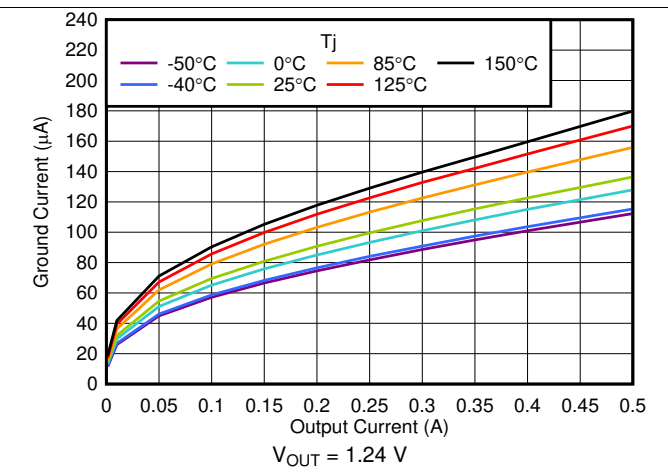
Figure 12. I_{GND} vs I_{OUT}
