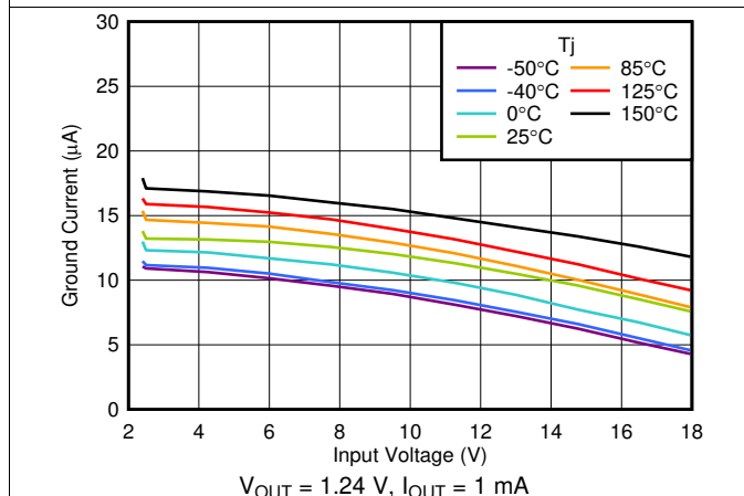
Figure 9. I_{GND} vs V_{IN}
