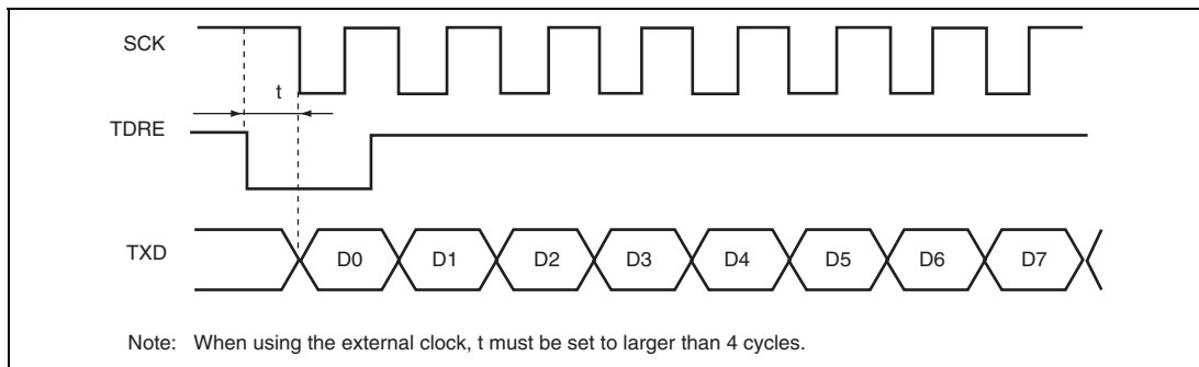
Figure 14.25 Example of Clock Synchronous Transfer Using DTC
