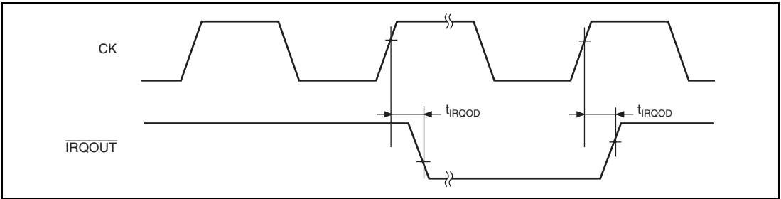
Figure 26.8 Interrupt Signal Output Timing
