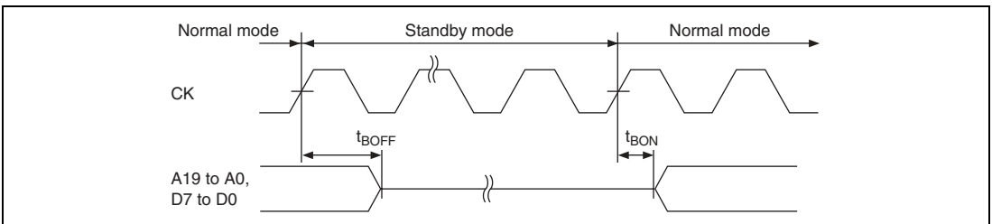
Figure 26.10 Pin Driving Timing in Standby Mode
