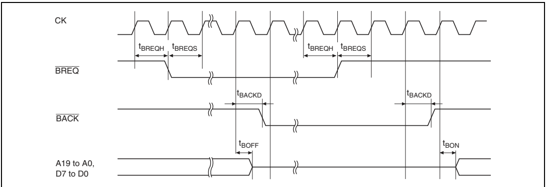
Figure 26.9 Bus Release Timing
