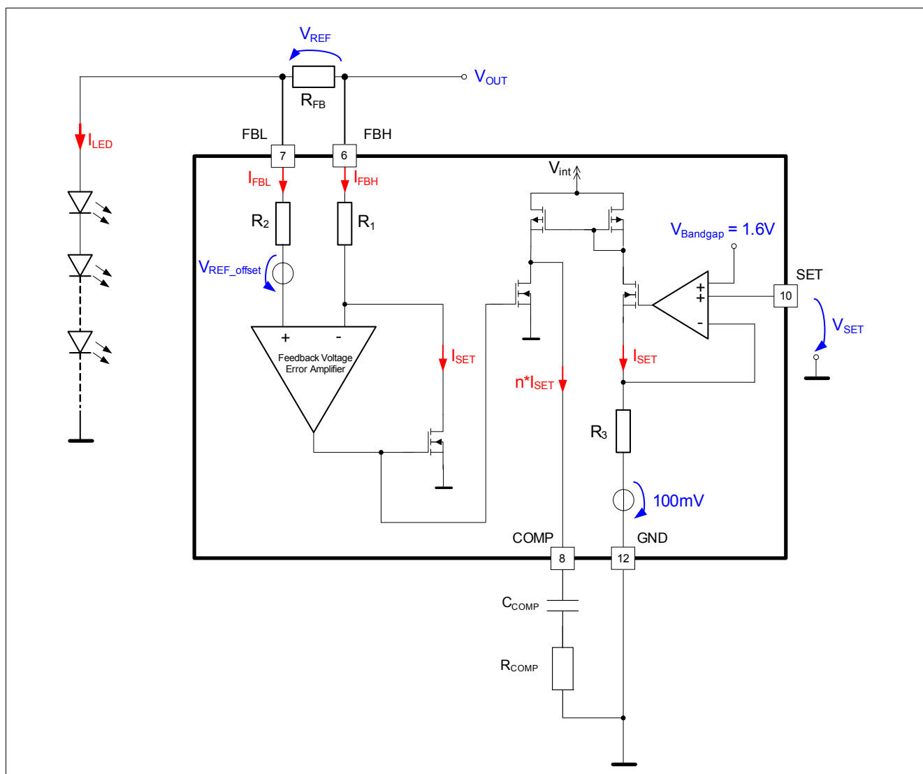
Figure 17 Concept Drawing Analog Dimming
