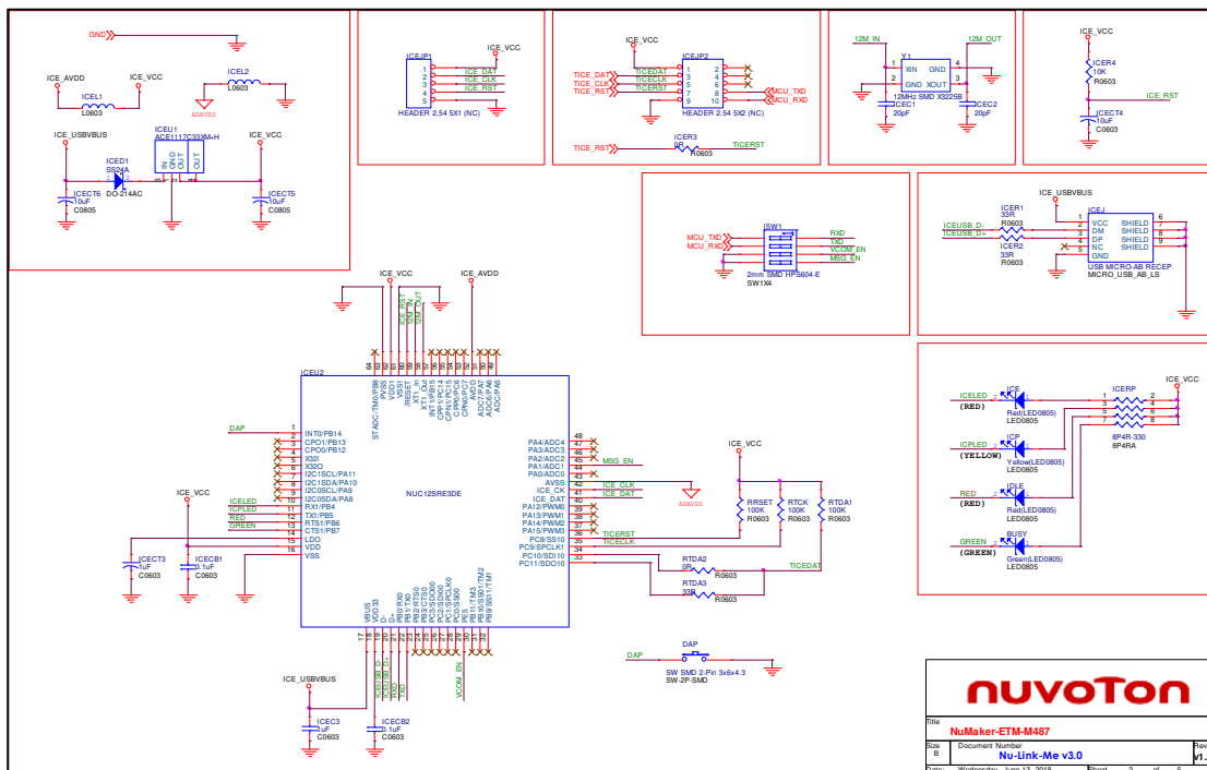
Figure 3-1 Nu-Link-Me Circuit
