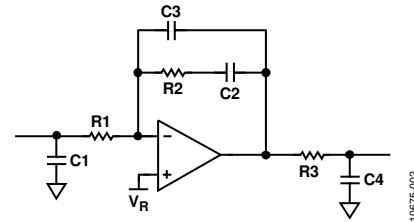
Figure 2. ADIsimPLL Filter
