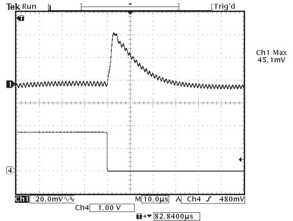
Figure 2 - Typical Transient Response, (Vin = 12 V, Output Current = 1.2 V), 7.5 A Load Step Change; Slew Rate = 200 A/μs Channel 1: Voltage Deviation = 45 mV; Recovery Time = 10 μs
