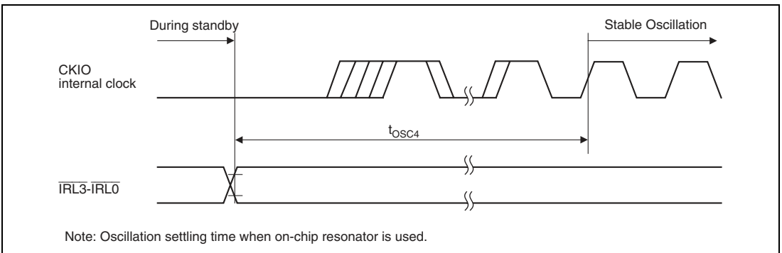
Figure 33.11 Standby Return Oscillation Settling Time (Return by \overline{\text{IRL3}} to \overline{\text{IRL0}} )
