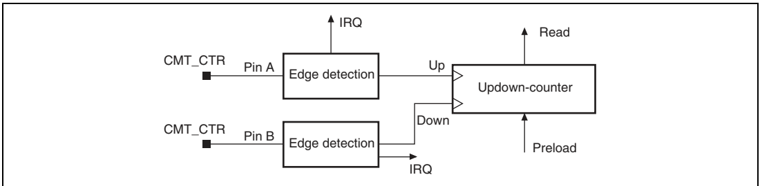
Figure 16.8 Updown-Counter Mode
