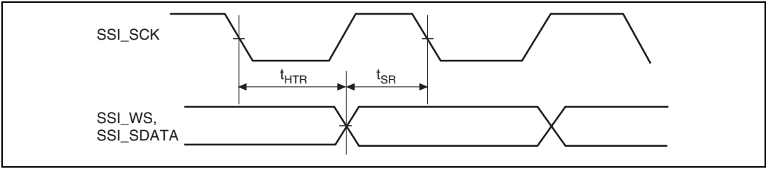
Figure 33.87 SSI Receive Timing (2)
