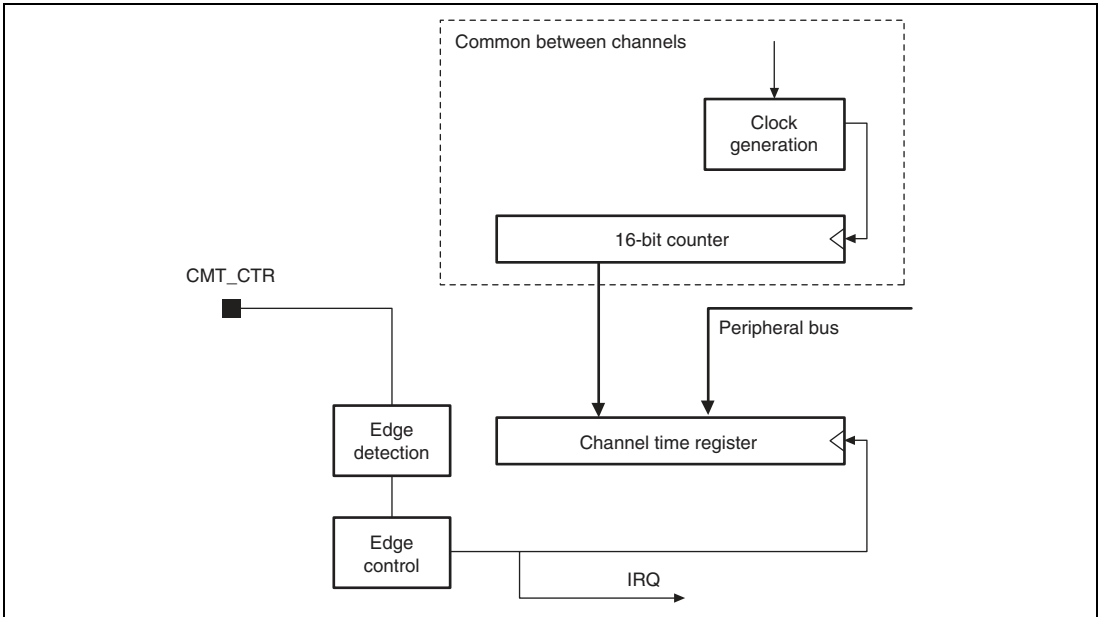
Figure 16.6 16-Bit Timer Mode: Input Capture
