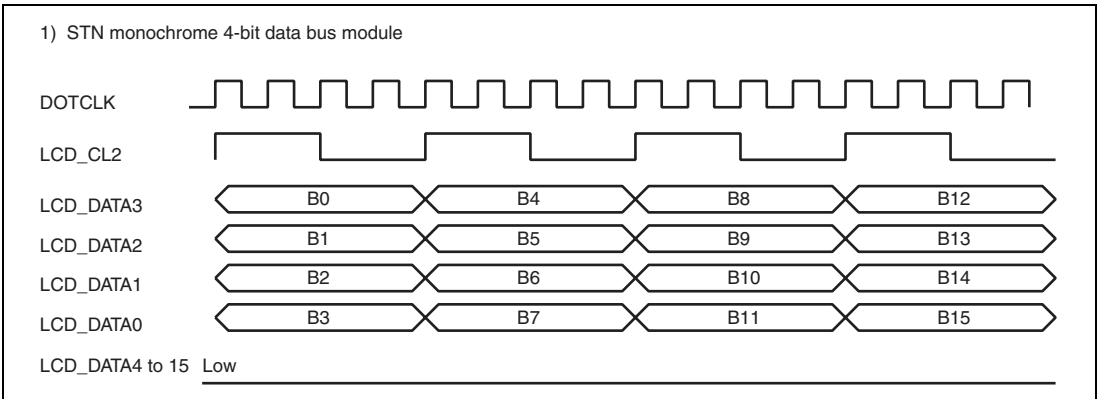
Figure 30.8 Clock and LCD Data Signal Example
