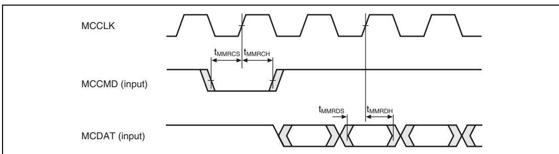
Figure 33.77 MMCIF Receive Timing
