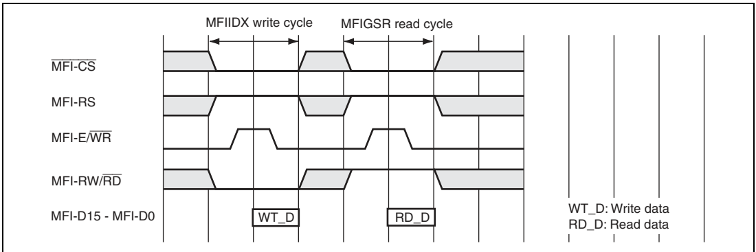
Figure 27.6 Writing to MFIIDX and Reading from MFIGSR
