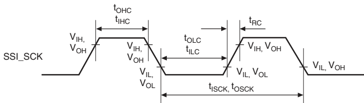
Figure 33.83 SSI Clock Input/Output Timing
