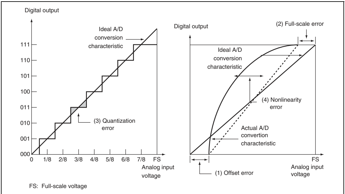
Figure 29.7 Definitions of A/D Conversion Accuracy
