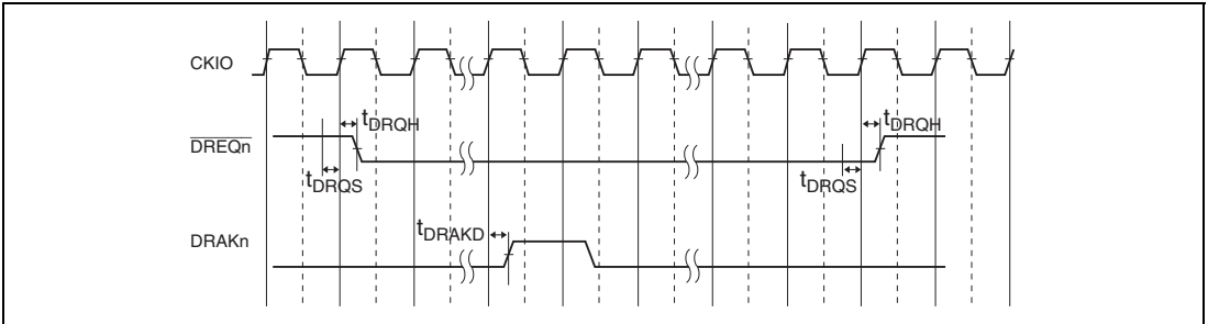
Figure 33.50 \overline{\text{DREQ}}/\overline{\text{DRAK}} Timing
