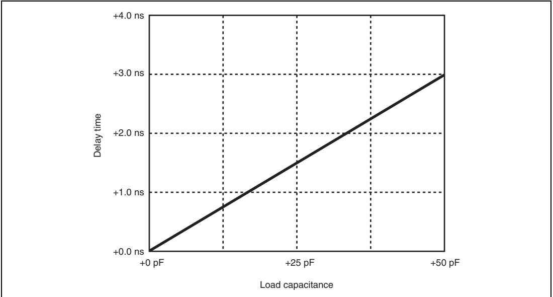
Figure 33.89 Load Capacitance-Delay Time
