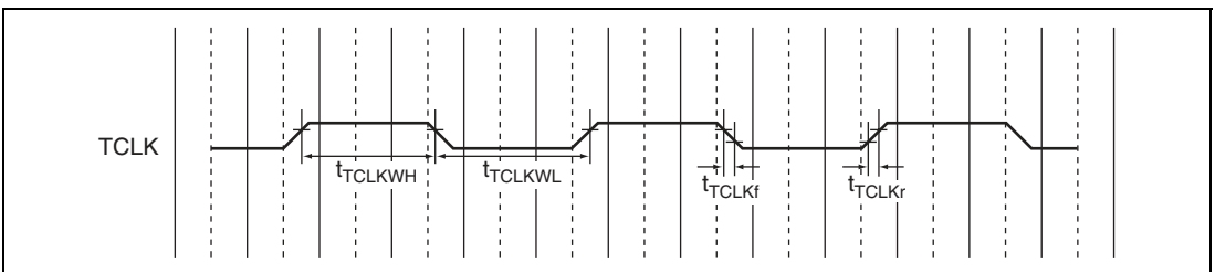
Figure 33.51 TCLK Input Timing
